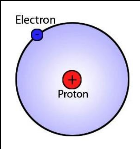
Hydrogen Atom
