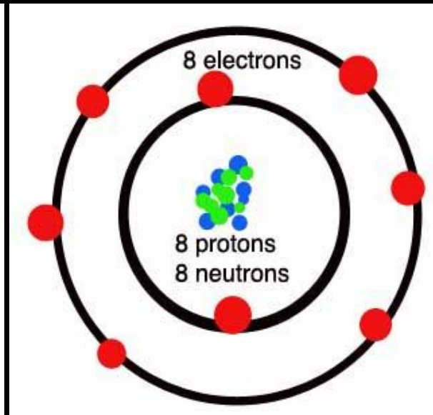
Oxygen Atom
