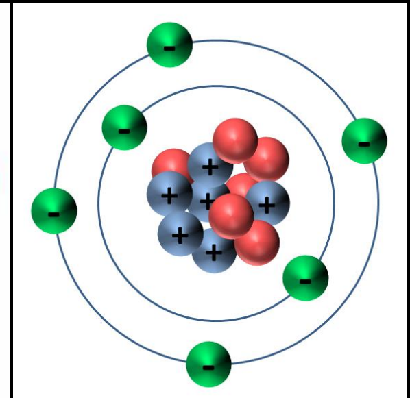
Carbon Atom
